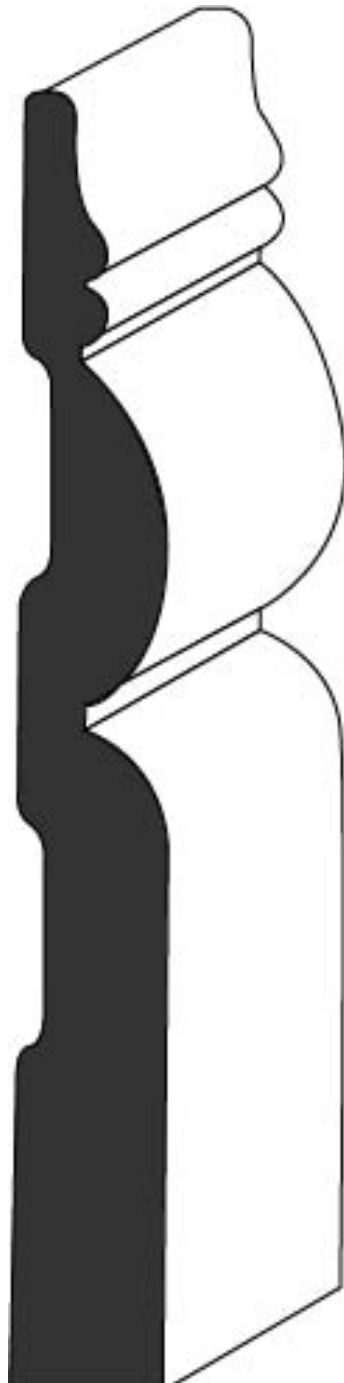
C-630 5/8" x 5 1/2"
