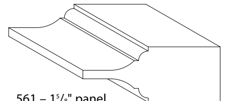
561 - 1 5 / 8 " panel
