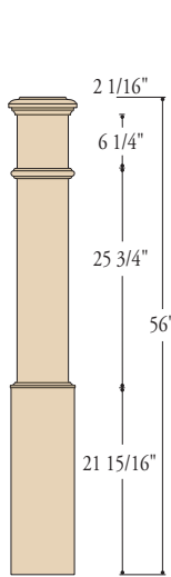
K-4095 7-1/2" X 56"
