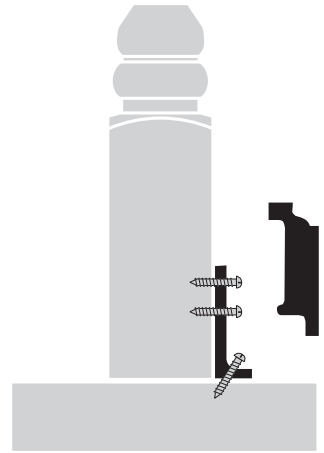
K-3505-30 - 3" K3505-35 - 3-1/2" L-Bracket Post Fastener
