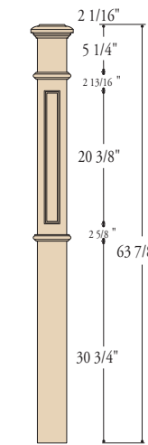
K-4691-FP 4-1/2" X 63-7/8"
