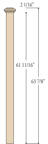
K-4077 3-1/2" X 63-7/8"
