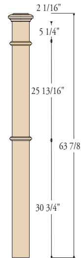
K-4695 4-1/2" X 63-7/8"
