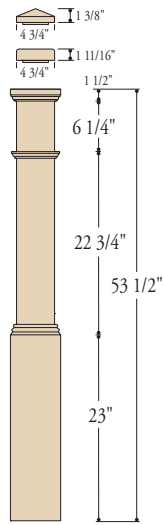
K-4091* 6-1/4" X 53-1/2"
