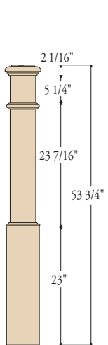
K-4090 6-1/4" X 53-3/4"
