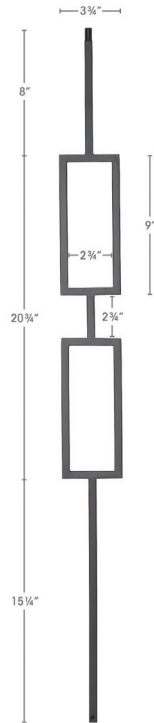
K-9091CS-44
