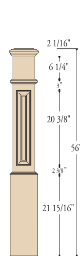
K-4891-RP 7-1/2" X 56"
