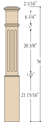
K-4095-F 7-1/2" X 56"
