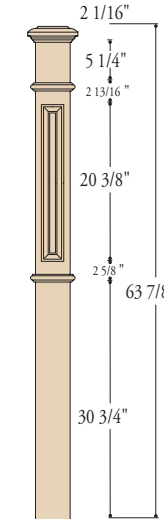
K-4691-RP 4-1/2" X 63-7/8"
