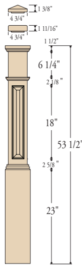
K-4091-RP* 6-1/4" X 53-1/2"
