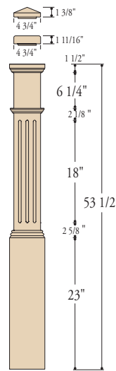
K-4091-F* 6-1/4" X 53-1/2"
