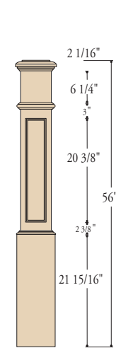
K-4891-FP 7-1/2" X 56"
