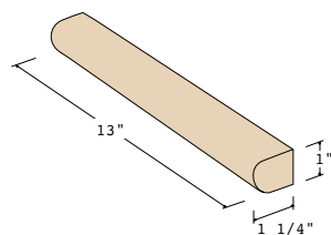
13" Return Nosing K-8080-13 1-1/4" x 1"
