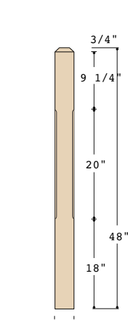
K-4002-C-48 3-1/2" X 48" STARTING
