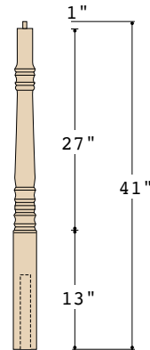
K-4272-RB 3-1/2" X 41" (O) VOLUTE (Round base, loose dowel)
