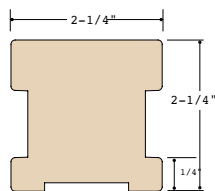
K-6350-ST-P 1-1/4" plow
