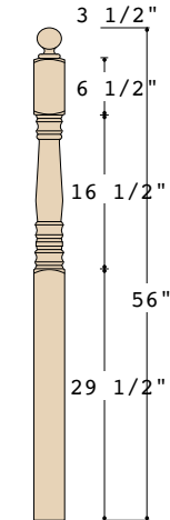
K-4504 3-1/2" X 56" (O) STARTING/LANDING
