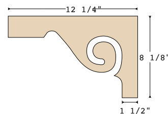
Tread Bracket K-8029 1/4" thick
