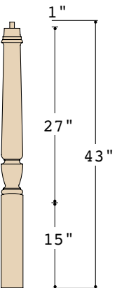
K-3010 3-1/2" X 43" (F, T) STARTING (Square Base)
