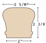
K-6210-ST
