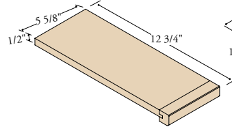
K-8072-2RE18 5-5/8" x 11-1/2"
