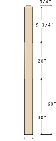
K-4002-C-60 3-1/2" X 60" LANDING
