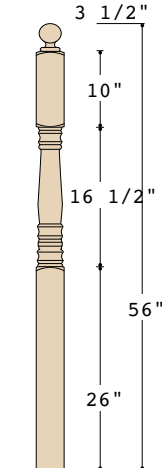
K-4503 3-1/2" X 56" (O) LANDING
