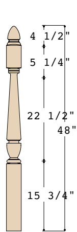
K-3030-ST 3-1/2" X 48" (F, T, O) STARTING
