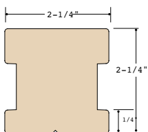
K-6350-ST
