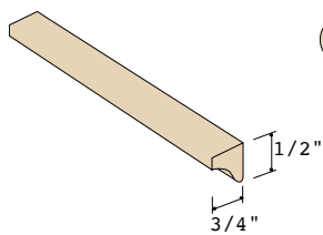
Cove Mould 1624-C 1/2" x 3/4"
