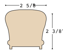
K-6210-ST-P1 1-3/4" plow
