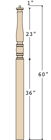
K-5515 3-1/2" X 60" (F, R, O) LANDING (Square Base)
