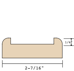
*K-6002-P1 1-3/4" plow
