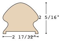
*K-6005-ST-P1 1-3/4" plow
