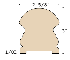
K-6519-ST-P1 1-3/4" plow
