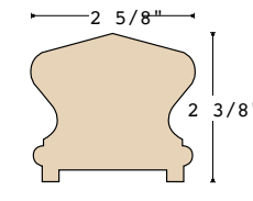
K-6910-ST-P1 1-3/4" plow
