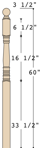
K-4304 3" X 60" STARTING/LANDING
