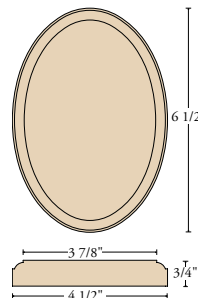
Rosette K-7337-L
