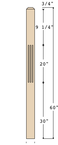
K-4002-F-60 3-1/2" X 60" LANDING
