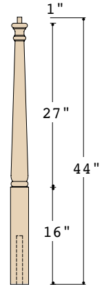
K-4061-RB 2-3/4" X 44" STARTING (Round base, loose dowel)
