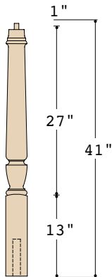
K-3012 3-1/2" X 41" (F, T) STARTING (Square base, loose dowel)
