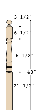
K-4500 3-1/2" X 48" (O) STARTING
