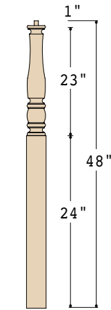
K-5511 3-1/2" X 48" (F, R, O) STARTING (Square Base)
