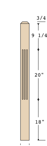
K-4002-F-48 3-1/2" X 48" STARTING
