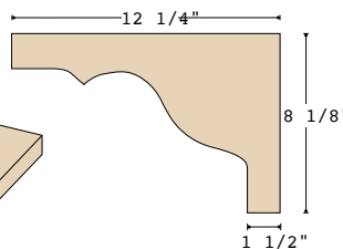
Tread Bracket K-8028 1/4" thick
