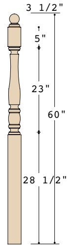
K-5560 3-1/2" X 60" (F, R, O) STARTING/LANDING
