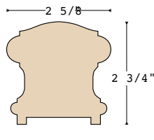
K-6710-ST-P1 1-3/4" plow
